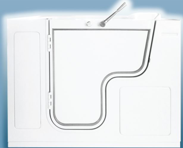
Model OH-5335 Outswing Door 53" x 35" x 37 \frac{1}{2} " Bariatric Tub. 30" wide seat.
